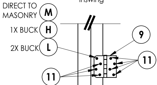
HINGE DETAIL Inswing
