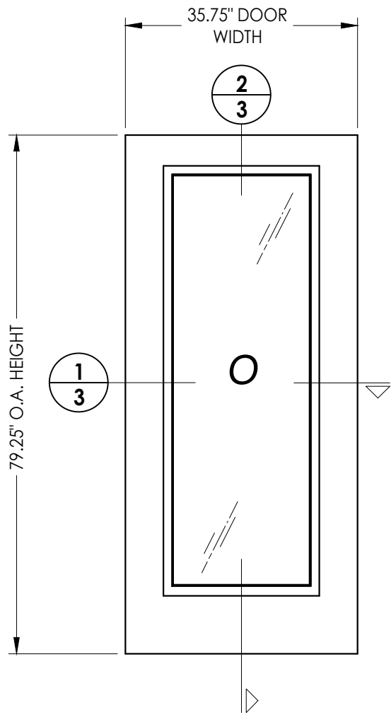
50 SIDELITE PANEL
