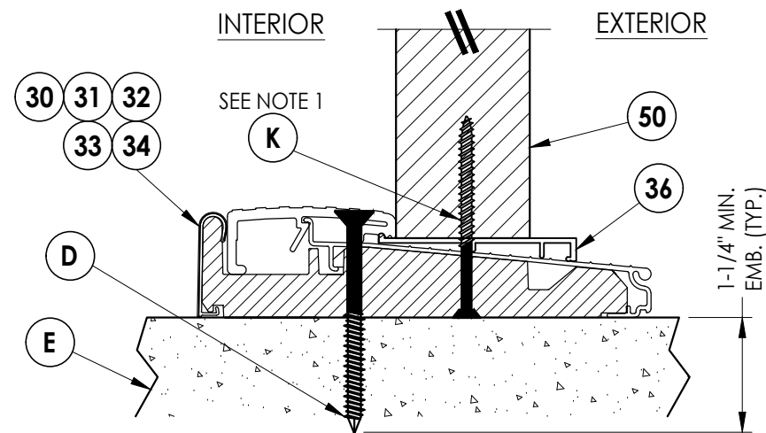
5 10 VERTICAL CROSS SECTION Outswing shown
