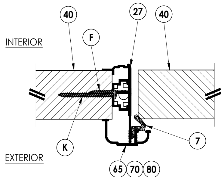
3 HORIZONTAL CROSS SECTION 6 Outswing shown - Inswing also approved
